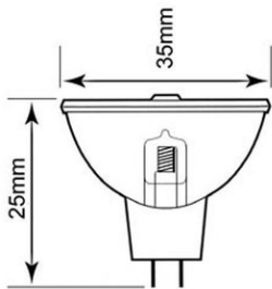
MR11
